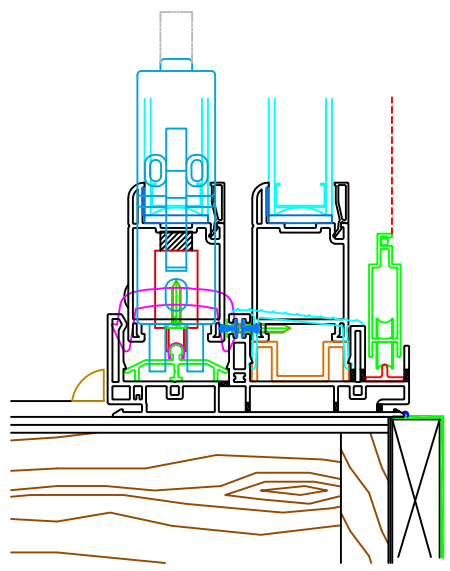
Patio Door Side View
